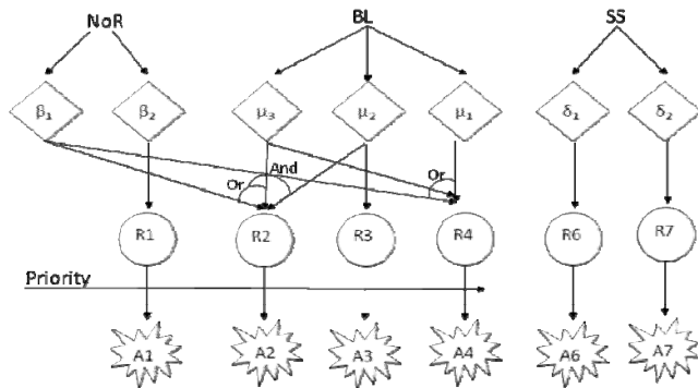
Figure 2. The Rule-Based Inference Engine of the PSM
